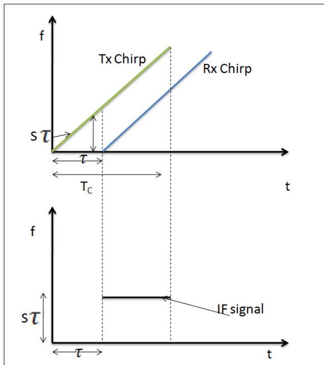
FIGURE 7: IF signal
