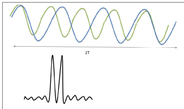
FIGURE 10: Sufficient observation window
