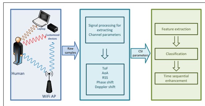
FIGURE 19: The general structure of CSI-based human behaviour sensing
