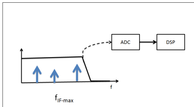
FIGURE 17: IF signal digitizing process
